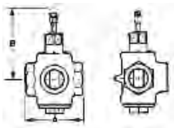
200L, 200T - Sizes 1/2" to 2" >4" size has bolted cover
