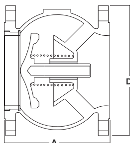
Single Check Valve Fig. 761
