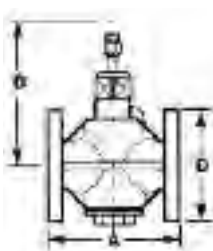
401M - Sizes 2" to 4"
